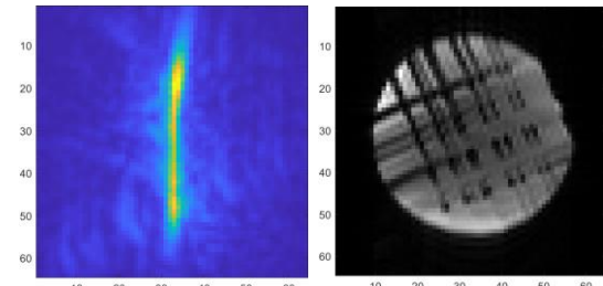
Fig. 2: Hybrid k-space data (left) and reconstructed SPEN-SE-EPI image (right) acquired by using the external gradient hardware to generate the quadratic phase profile for encoding.
