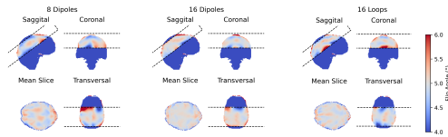
Fig. 3: Global excitation of 2-spokes in the motor cortex and mean flip angle distribution in slab-relative z direction for all coils.
