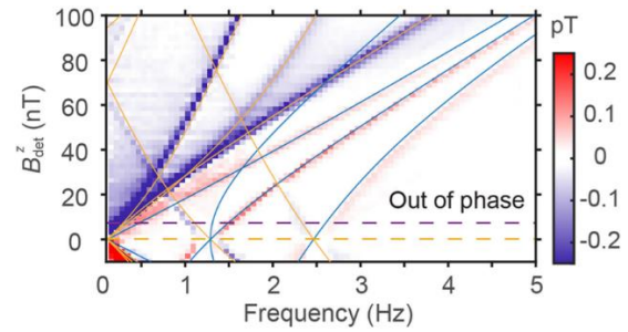
Fig. 5: Measured out of phase spectra as a function of the detection field B_{\text{det}} .
