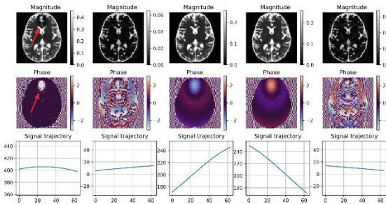
Fig. 5: Individual states of a bSSFP simulation. The left column shows magnitude and phase of the full reconstruction, with a banding artifact produced by B0 inhomogeneities (arrow). The remaining columns show states with \tau dephasings of -2, -1, 0 and 1 times TR.
