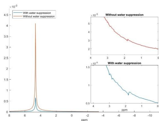
Fig. 3: Non-localized ^1\text{H} -MR spectra of the model solution acquired with our implementation of the FID sequence with and without WT WS, with identical and optimized shimming. The water signal was reduced by a factor of 6.
