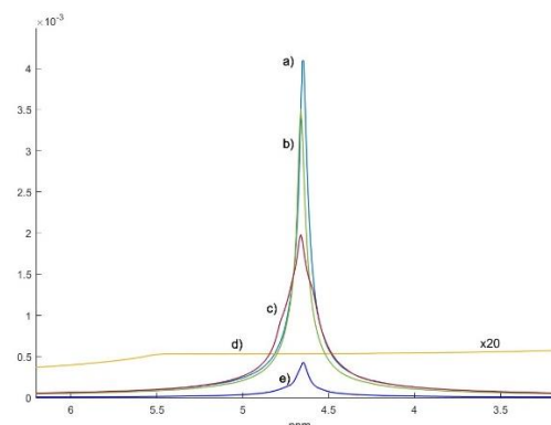
Fig. 1: Magnitude non-localized 1H-MR spectra of the spherical model solution: (a) our implementation,
