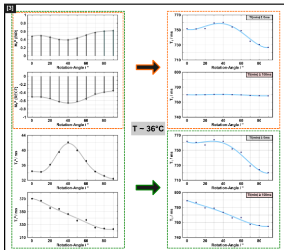
Fig. 5: Overview of anisotropic BSB model parameters as a function of \theta_{FB} (left column), obtained from the analyses illustrated in Figure 4 and resulting orientation-dependent T_1 (right column) from fits to the simulated IR data.
