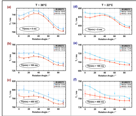
Fig. 2: Apparent spin-lattice relaxation times obtained from monoexponential fitting of IR curves measured with hard-pulse inversion ( \tau_p=40 \mu\text{s} ) at 36 °C (a–c) and 22 °C (d–f) as a function of the rotation angle.
