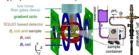
Fig. 1: Schematic diagram of the ULF MR system. Freshly produced parahydrogen (pH 2 ) is supplied to the sample container inside a magnetic shield.
