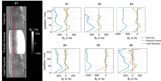
Fig. 1: Field maps before (Tune-Up) and after B_0 shimming (Pseudo Inverse and Least-Squares) in the first subject (left) and the median B_0 along the T/L-Spine (right) in all six subjects.
