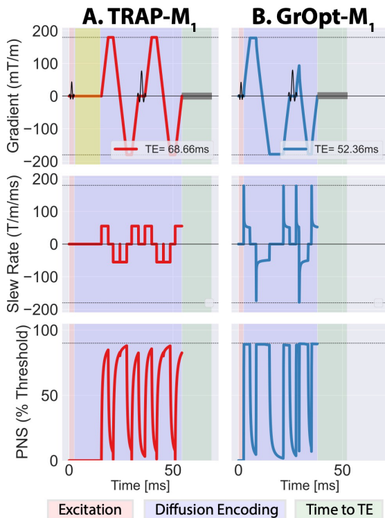
Fig. 1: (A) TRAP-M 1 vs. (B) GrOpt-M 1 waveform. TRAP waveforms have unused time (yellow) to allow for moment nulling while GrOpt utilizes the full slew-rate, avoids PNS and fulfills other constraints.
