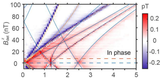
Fig. 4: Measured in phase spectra as a function of the detection field B_{\text{det}} . The solid lines indicate the simulated position of resonances. Dashed lines indicate the position of the spectra in Fig. 6.
