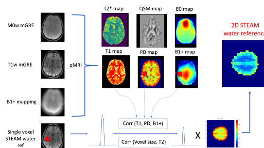
Figure 1: Overview of the proposed method for water referencing using single voxel STEAM and mp-qMRI. The water reference intensity measured using STEAM is corrected for B1+, PD and T1 with values from qMRI. Multiplying the PD map with the corrected STEAM water signal provides a water reference image with spectroscopic metrics, i.e., scaling refers to assumed water intensity at any voxel.
