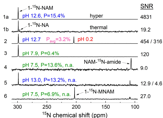
Fig. 1: pH dependent behavior of 1\text{-}^{15}\text{N} -nicotinamide, -nicotinic acid, and -methyl nicotinamide. One can see that when neutralizing pH after the transfer (3) only little signal is retained compared to basic pH (1). If \text{D}_2\text{O} instead of \text{H}_2\text{O} is used, a common method to prolong T_1 of hyperpolarization, no signal of the 1\text{-}^{15}\text{N} is retained. If naturally abundant methyl nicotinamide is used, where the \text{CH}_3 -group protects the 1\text{-}^{15}\text{N} , polarization is retained and the T_1 is over 200 s long.
