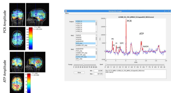
Fig. 1: Exemplary 31P MR spectrum and metabolite maps for PCr and ATP. ATP: Adenosintriphosphate; PC: Phosphocholine; GPC: Glycerophosphocholine; PCr: Phosphocreatine; PE: Phosphoethanolamine; GPE: Glycerophosphoethanolamine; NADH: Nicotinamide adenine dinucleotide oxidized.
