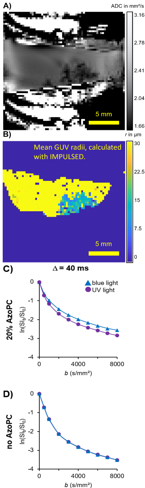
Fig. 2: A) ADC map of GUVs in Eppendorf tube and (B) pixelwise fit of IMPULSED radii. Signal changes within the GUV patch relative to b_0 under UV light (purple) and blue light (blue) ( \delta = 7 ms) for GUVs with (C) and without AzoPC (D).
