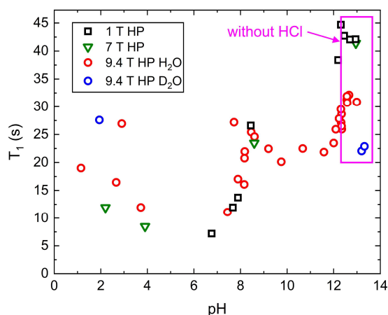
Fig. 2: This figure demonstrates the volatility of hyperpolarized 1\text{-}^{15}\text{N} -NAM T_1 values depending on pH. Basic pH (without HCl added) was used for imaging.
