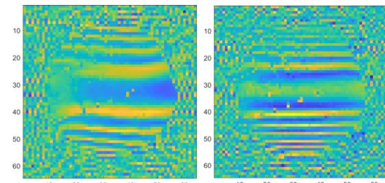
Fig. 3: Quadratic phase profile of the reconstructed images using the external gradient hardware for the generation of the quadratic phase profile (left) and using the chirp RF pulse method (right).
