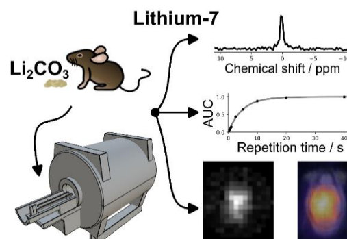
Figure 1: In vivo 7 Li MRI and MRS were acquired from mice on a lithium-enriched diet. Weekly 7 Li MRS was performed to monitor the uptake of lithium and to estimate the T1 relaxation time. 4-hour SPIRAL 7 Li MRI was at a resolution of 2×2×3 mm 3 . [Reproduced from Memhave et al. 16 ]
