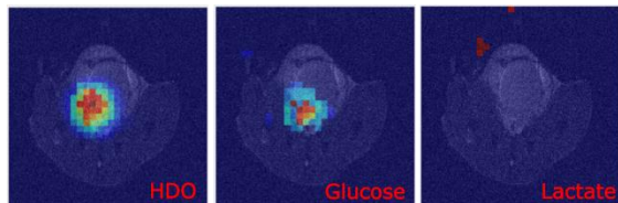
Fig 2: 2 H image of H 2 O, Glucose and lactate in a colitis model at day 8, acquired with FID-CSI. Averages=20, TR=250 ms.
