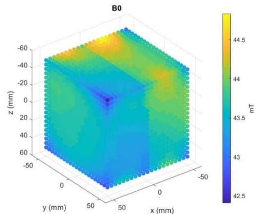
Fig. 3: Magnetic field of a Halbach magnet, whereby an average magnetic field of B_0 = 43.75\text{mT} , an overall homogeneity \Delta B = 5.5\% were measured. The jump at \Delta x = 5\text{mm} is due to a restart of the sensor.
