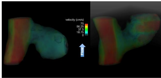
Fig. 4: Volume rendering of the peak flow through the vessel phantom (pulsatile mode). Two different connection directions were examined.
