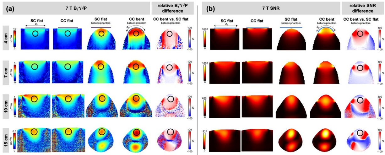
Fig.7: 7 T MRI results, (a) B_1+/-P maps and (b) SNR maps in the central sagittal slice for the 4, 7, 10 and 15 cm SC and CC in flat position and the SC in flat and the CC in bent position, relative B_1+/-P and SNR difference maps (CC vs. SC on balloon phantom).
