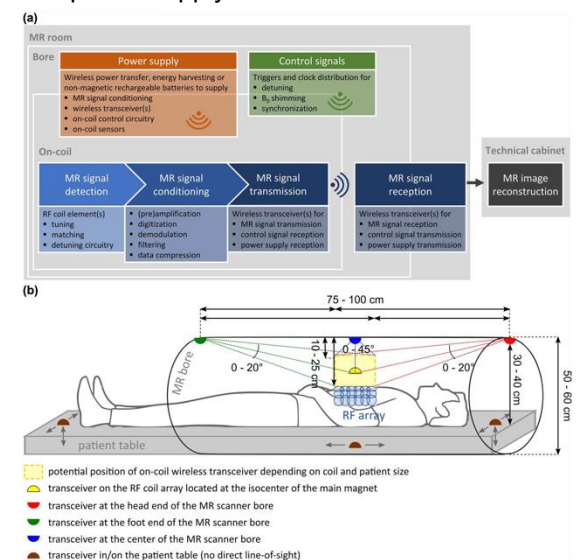
Fig.8: (a) Functional block diagram of a wireless MR receive chain consisting of three main subsystems: wireless MR signals (blue), control signals (green), and power supply (orange). (b) Side view of wireless transceiver positioning variants.
