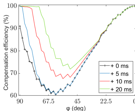
Fig. 3: Compensation efficiencies for the angle interval \phi = [90, 0]^\circ between the two waveforms for an increase of the waveform duration between 0 and 20 ms.
