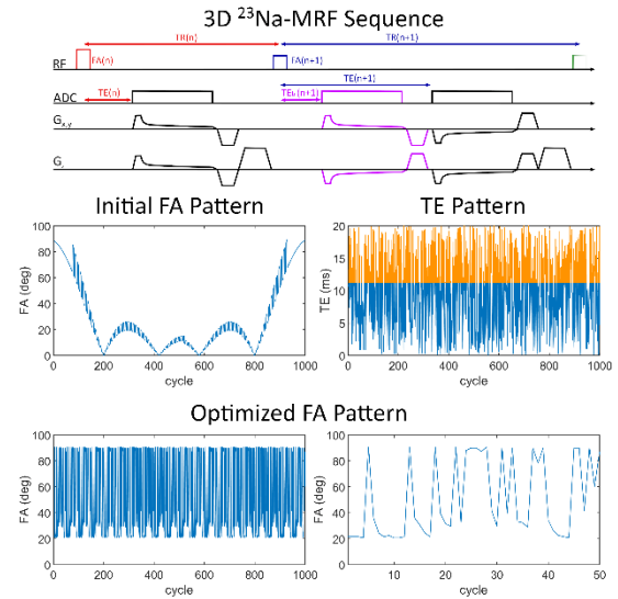
Figure 1: 3D ^{23}\text{Na} -MRF sequence diagram, where the purple readout is inserted in the MRF II sequence if TE is larger than the time required for acquisition of a spoke. TEs for which this holds true are marked in orange in the TE pattern. The initial (MRF I) and the optimized (MRF II) FA pattern are shown.
