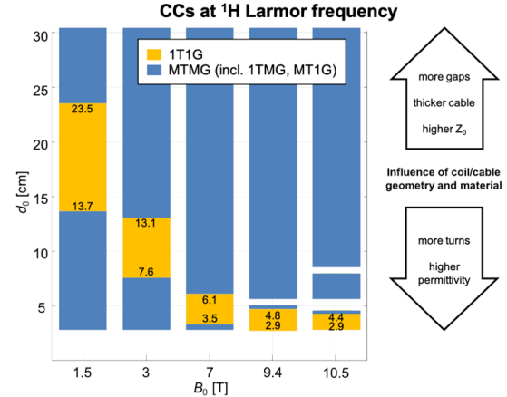
Fig. 2: Possible coaxial coil (CC) diameters ( d_0 ) at the ^1\text{H} Larmor frequency for 5 different common field strengths using realistic coil and cable parameters.
